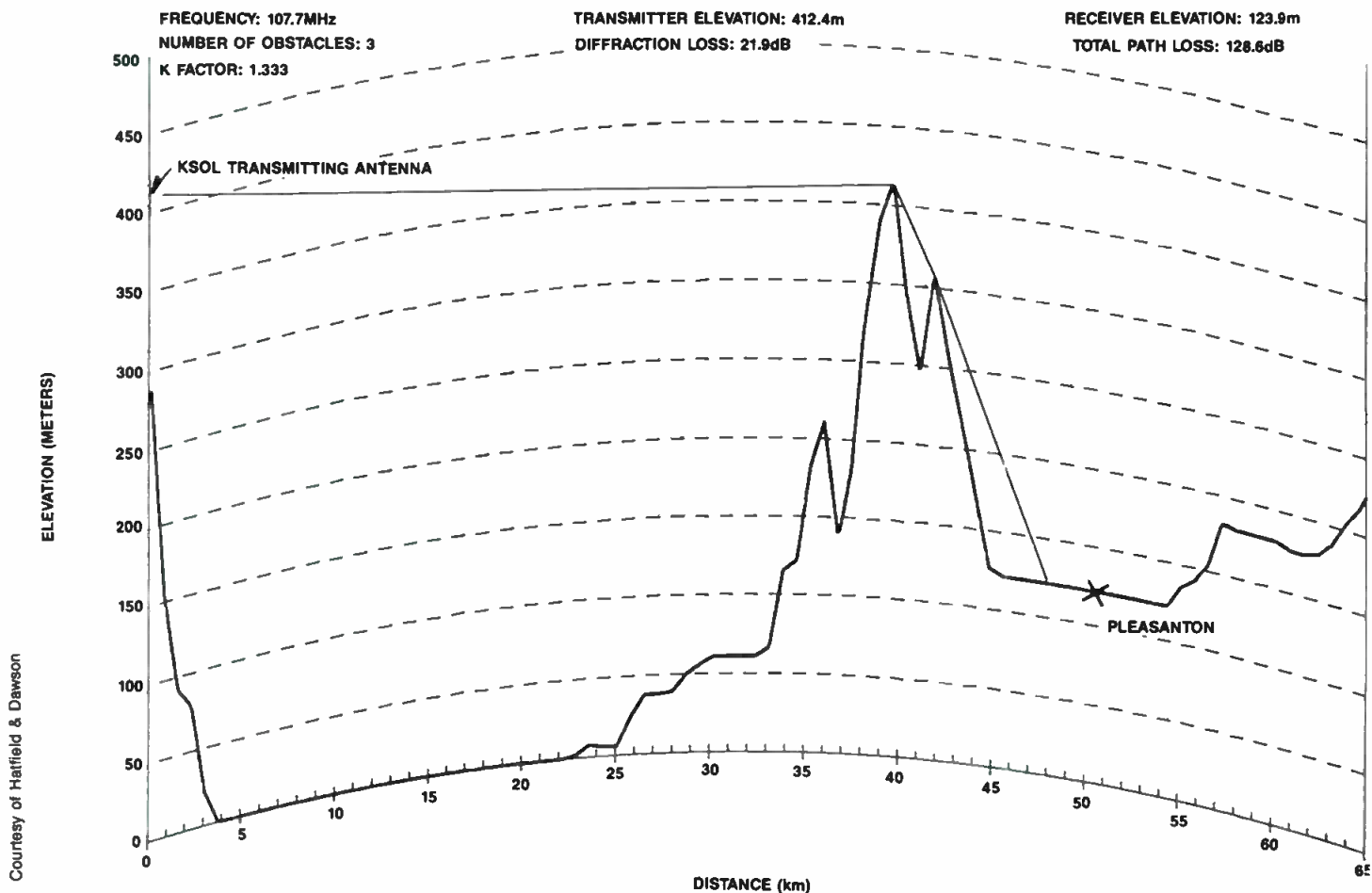
Figure 2. Elevation plot of the San Francisco Bay area showing the signal blockage suffered by KSOL-FM (and many other Bay area broadcasters). The mountain ridge effectively shields the community of Pleasanton from service, despite predicted Grade A coverage signal strength.
