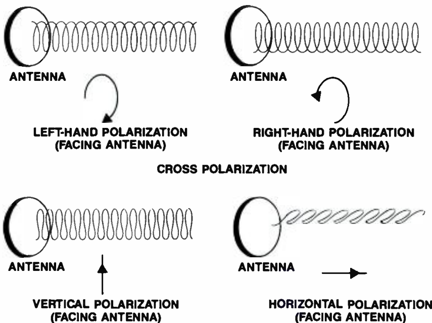
Figure 1. Four different polarizations. Polarization of receive antenna must match transmit antenna. Alternate transponders use opposite polarizations to perform "frequency reuse."
