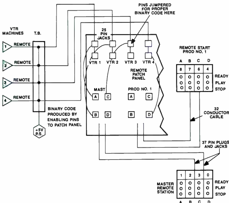
Figure 1. The VTR remote-control system relies on a patchbay arrangement, allowing any machine to be controlled from any location.
