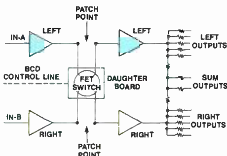
Figure 2. Stereo distribution amplifier card. Each channel's signal path is interrupted after the input buffer, but before the output line driver. An optional daughterboard, controlled via BCD signals, permits the audio to be specially configured to stereo, inverted polarity, mono sum or matrixed.
