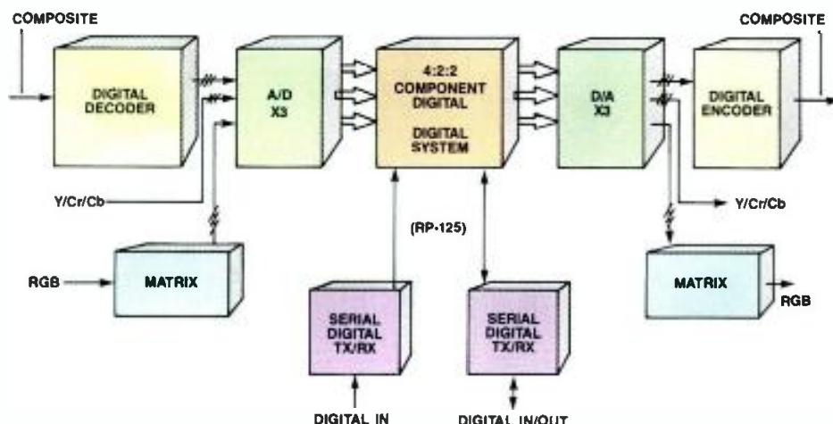
Figure 1. The component digital device accepts input and makes output in several formats, including composite video via a decoder/encoder. Internally, the device processes component video based on a 4:2:2 ratio.
