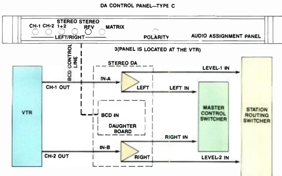
Figure 3. Signal and control flow for the stereo channels of a typical 2-channel program source.
