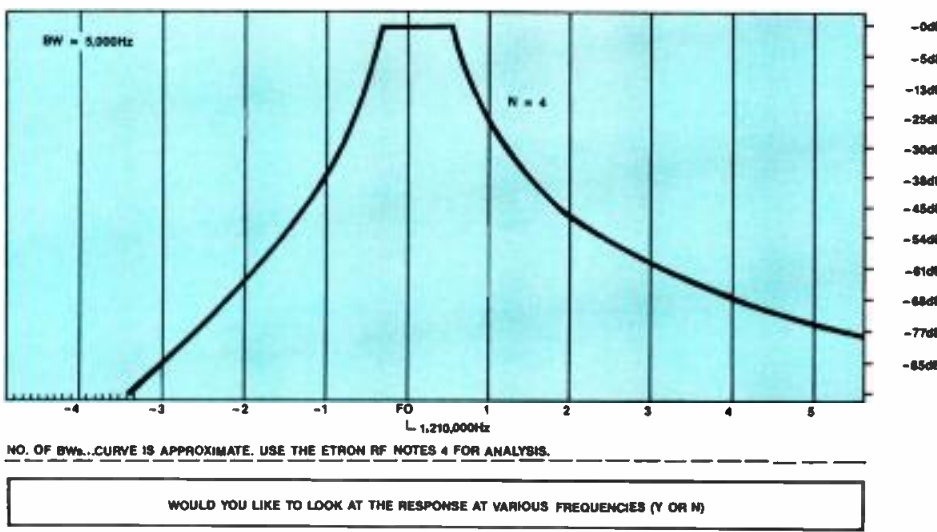
Figure 5. Insertion loss for circuit calculated in Figure 4.
