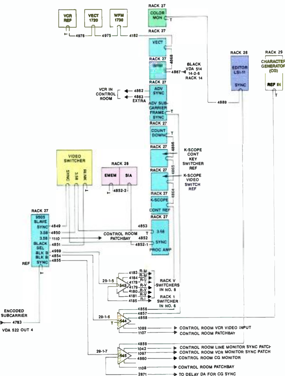
Figure 1. At the foundation of any new design or upgrade are the pulse and signal-flow diagrams. These diagrams should include cable and equipment location numbers to reduce confusion and help in equipment setup.
