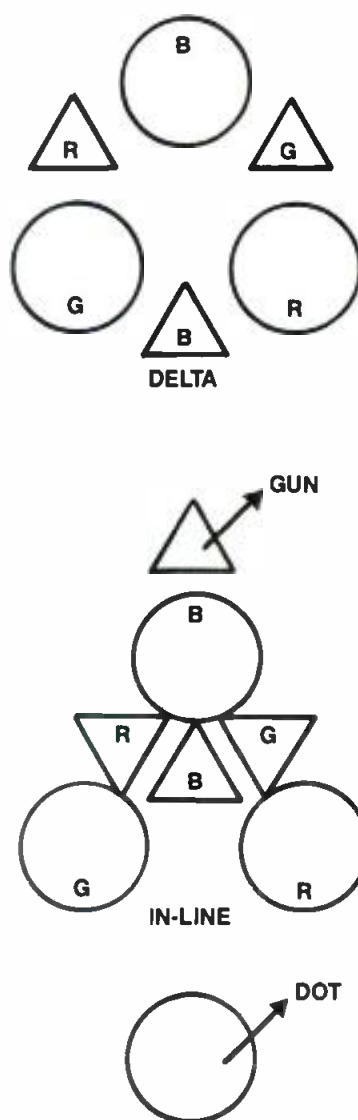
Figure 1. Geometries of the two dot-mask type CRTs.
